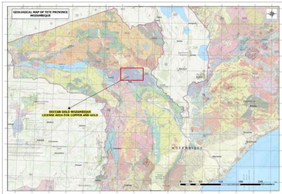
Figure 2: Location of copper exploration area within the Tete Complex of Central-West Mozambique
