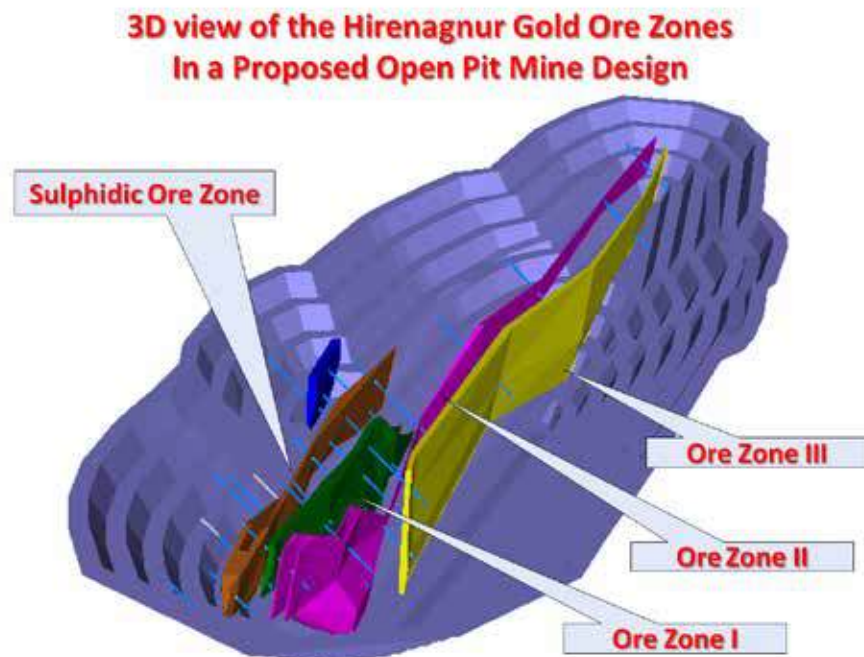
Fig-21 : 3D view of the Hirenaganur Gold Ore Zones and Open Pit Mine Design.
